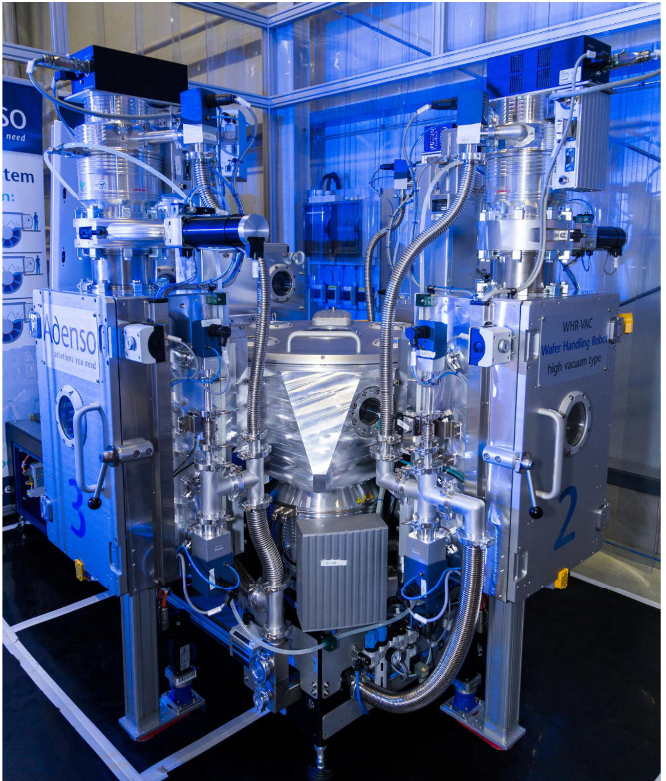
This pic showing: Adenso Waferhandling.Platform with central waferhandling module WHM, Load Lock Modules LLM, vacuum system adVAC , electronics and cluster control software adControl
